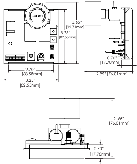
FIGURE 1: DIMENSIONS
