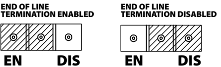
FIGURE 7: EOL TERMINATION JUMPERS
