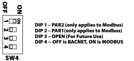
FIGURE 6: SW4 DIPSWITCH SETTINGS
