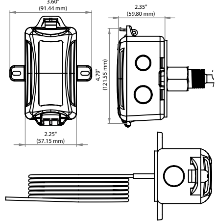
FIGURE 1: ENCLOSURE DIMENSIONS
