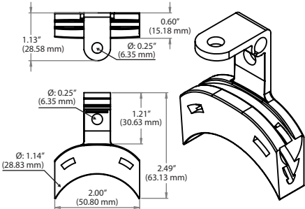
FIGURE 4: MOUNTING CLIP DIMENSIONS
