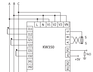
3 phase 3 wire (2LL, 3CT)
