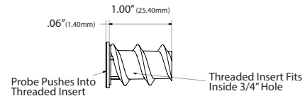
Spacers / Anchors
